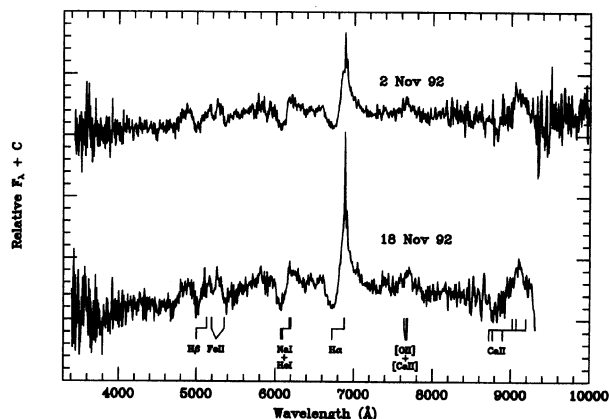
FIG. 2. Spectroscopic observations of SN 1992am during the nebular phase. The observations are not corrected for the redshift of the host galaxy, 14\,600\text{ km s}^{-1} .
