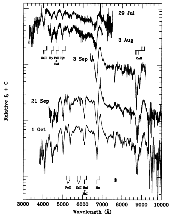
FIG. 1. Spectroscopic observations of SN 1992am during the photospheric phase. The observations are not corrected for the redshift of the host galaxy, 14\,600\text{ km s}^{-1} .
