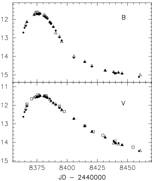
FIG. 6.—Comparison of our B and V light curves of SN 1991T (circles) with the preliminary photometric reductions of the CTIO data published by Phillips et al. (1992) (triangles). The V magnitudes from the Van Vleck Observatory study by Ford et al. (1993) are plotted as squares.
