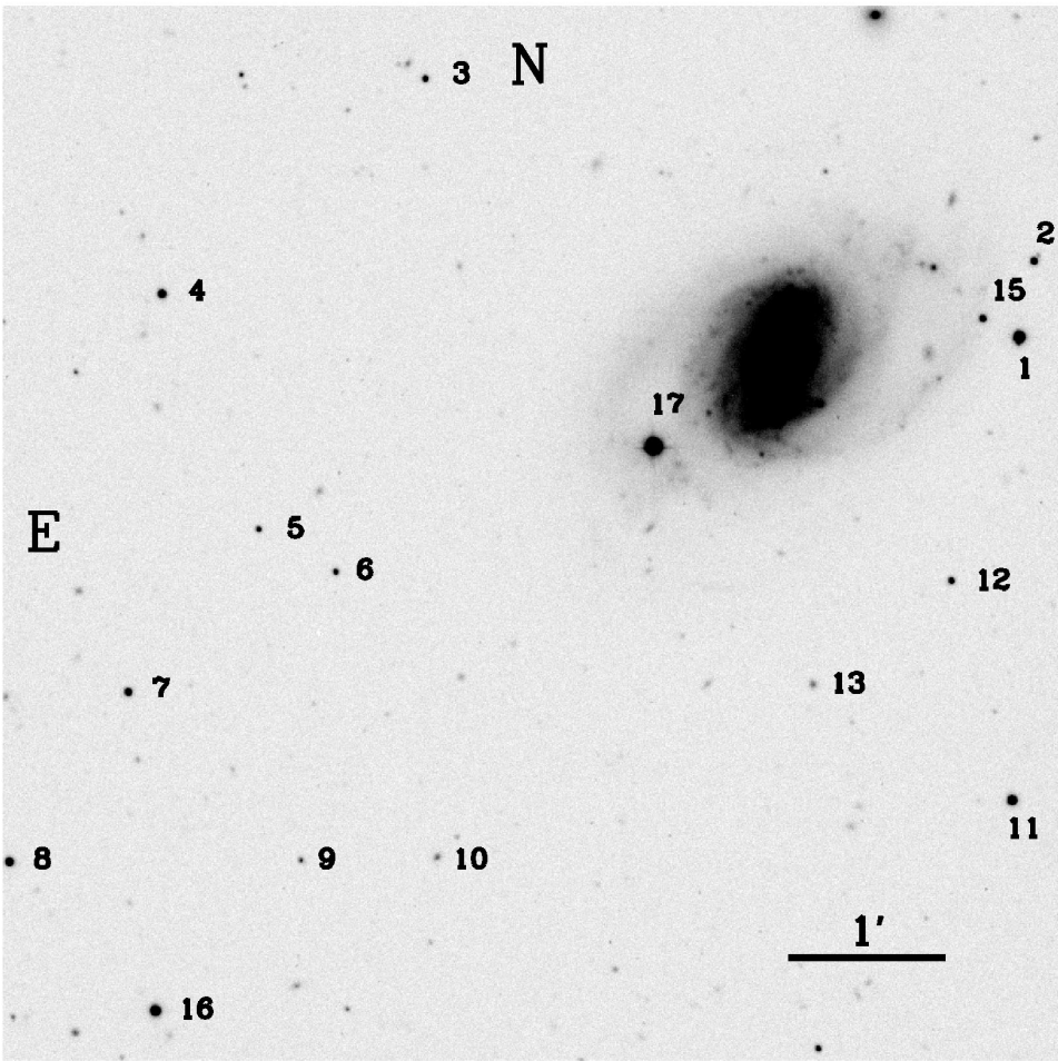
FIG. 1.—SN 1990N in NGC 4639. The local standards listed in Table 3 are marked. This R image was taken at the CTIO 0.9 m telescope on 1994 March 13. The field is 6".8 on a side. Star 14 does not appear on this chart. It is located at (12 h 42 m 47 s .0, +13°17'52", J2000.0) on the Digitized Sky Survey.
