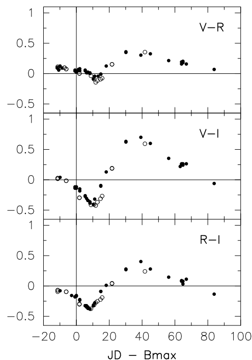
FIG. 11.—Observed V-R , V-I , and R-I color evolution of SN 1990N (open circles) and SN 1991T (filled circles) as a function of time since B_{\text{max}} .
