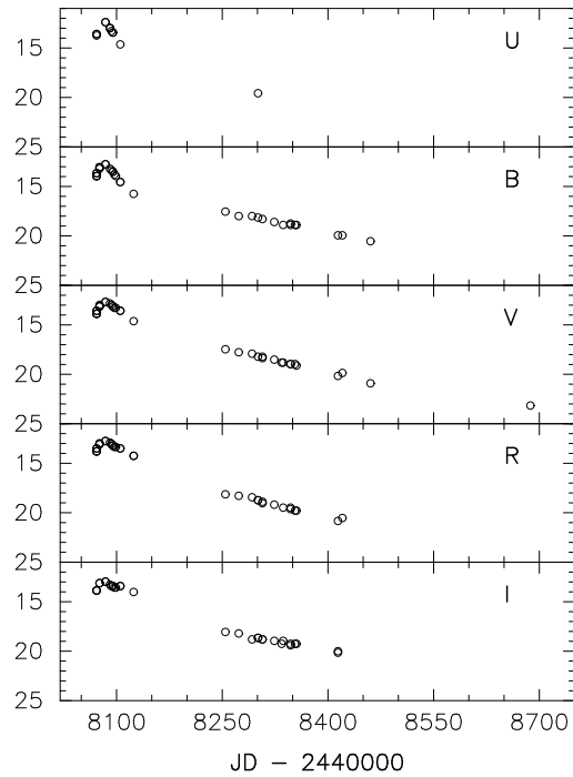
FIG. 3.— UBVR light curves of SN 1990N
