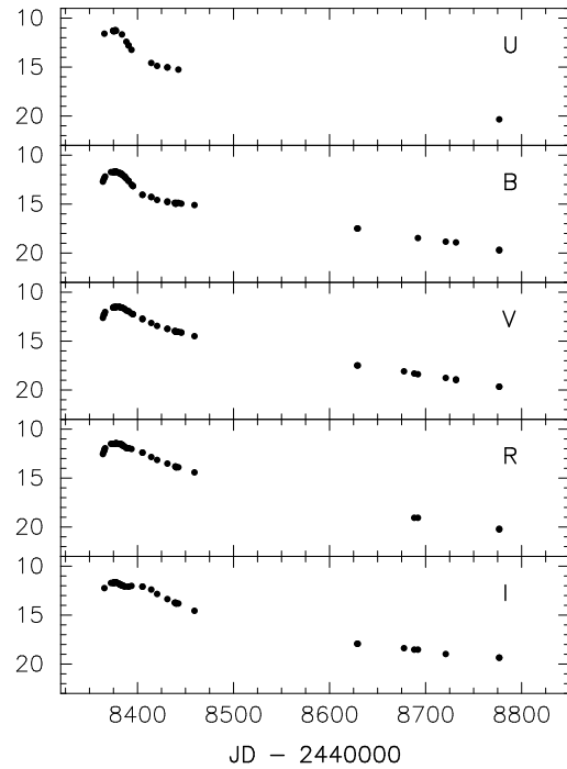
FIG. 4.— UBVR light curves of SN 1991T
